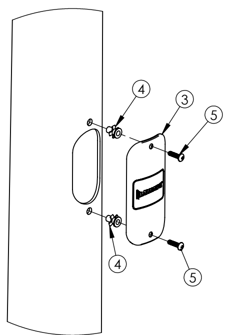
DETAIL A COVER ASSEMBLY SCALE 1 : 6
